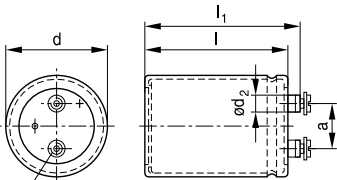
B43564 Ring clip/clamp mounting
