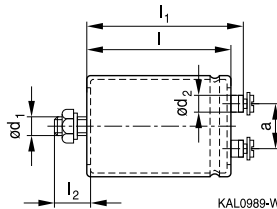
B43584 Threaded stud mounting
