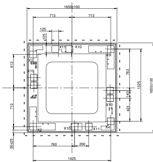
all dimensions in µm
