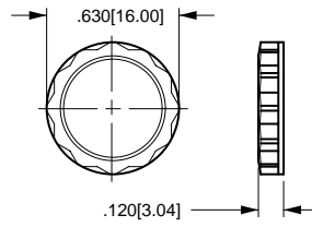
PLASTIC FACENUT (Fits 9/16" and 14mm wrenches) .630" X .120" [16.00] X [3.04] BLACK - 384-17131
