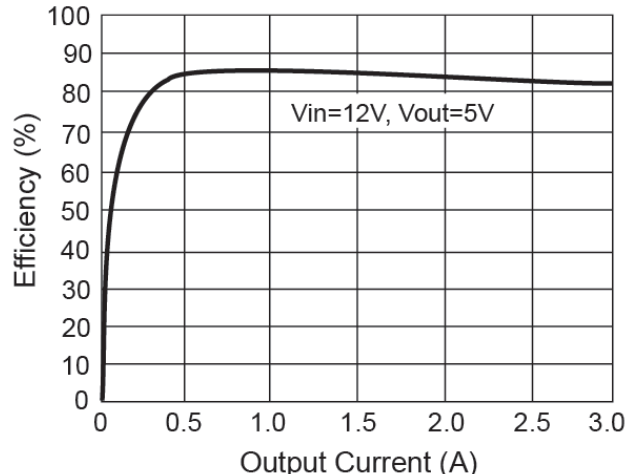
Figure 6. Efficiency
