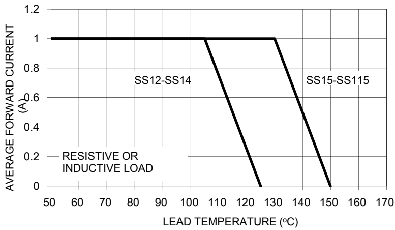
FIG.1 FORWARD CURRENT DERATING CUURVE
