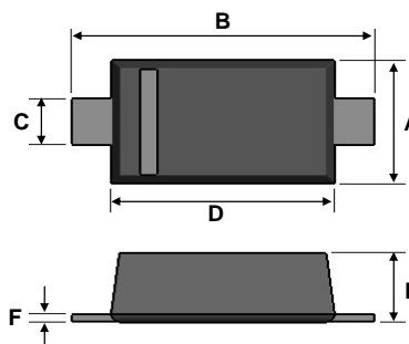
SOD-123F
